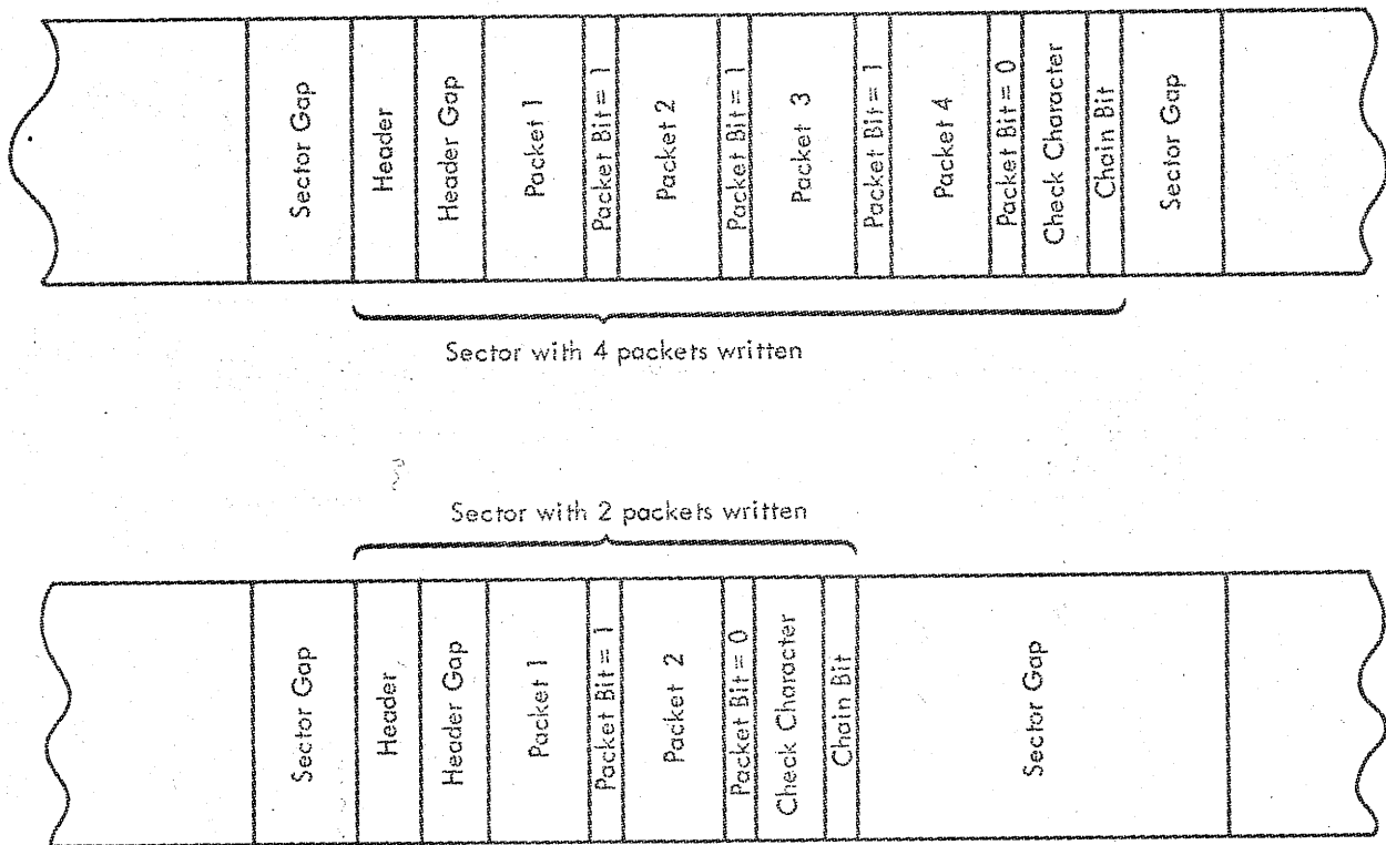
Figure 7. Organization of a Sector
