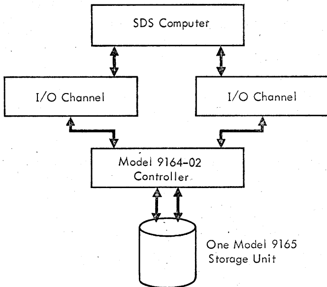
Figure 3. One SDS Computer with Dual Operation of File Storage Unit
