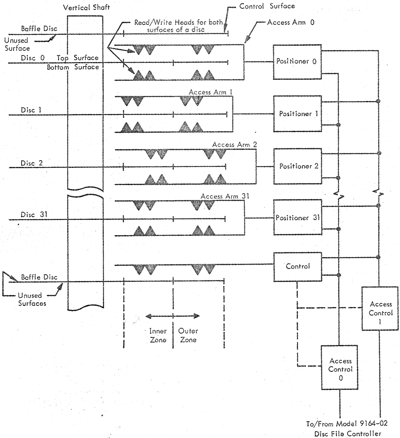
Figure 5. SDS Model 9165-24 Disc File Storage Module
